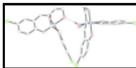
Fig. 2. The crystal packing of the title complex, viewed along the c axis. Hydrogen bonds are shown as dashed lines.
