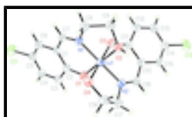
Fig. 1. The molecular structure of the title complex with 30% probability displacement ellipsoids.
